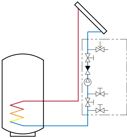
LK 211 SOLARSTATION S WITHOUT CONTROLLER
