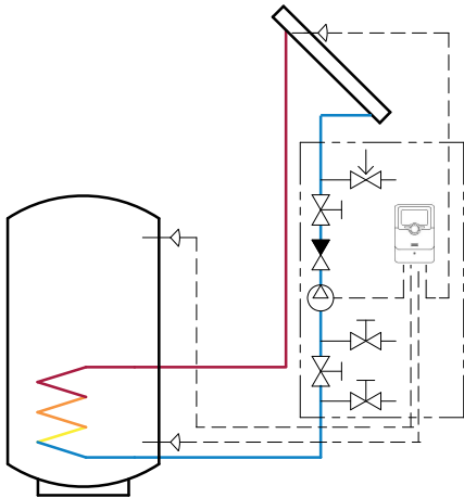
LK 211 SOLARSTATION S WITH LK 152 SMARTSOLAR SLL
