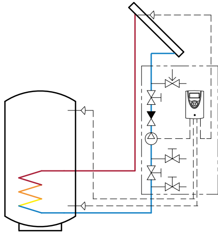
LK 211 SOLARSTATION S WITH LK 152 SMARTSOLAR SC PLUS
