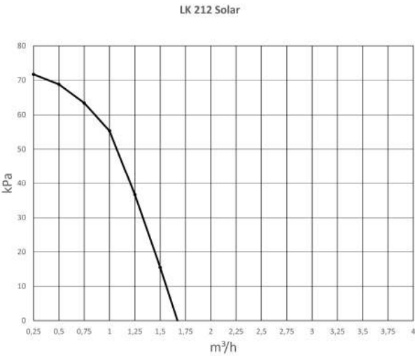
CAPACITY DIAGRAM
