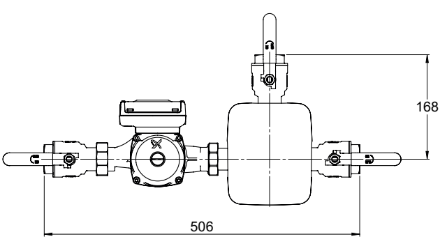
LK 815 - 1¼" FEMALE THREAD
