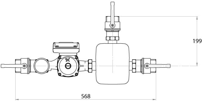
LK 815 - 1½" FEMALE THREAD
