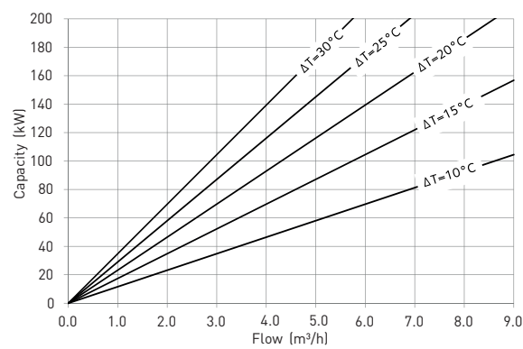
BOILER CAPACITY DIAGRAM
