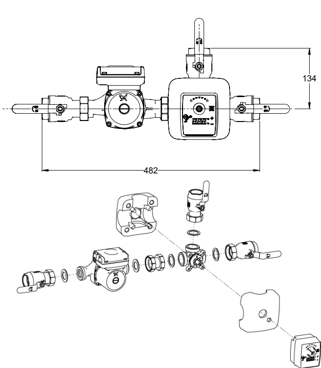
LK 816 - 1¼" FEMALE THREAD
