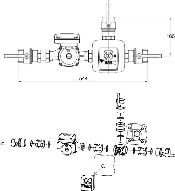
LK 816 - 1½" FEMALE THREAD
