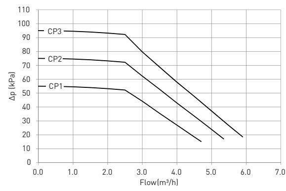
PUMP CHARACTERISTICS
